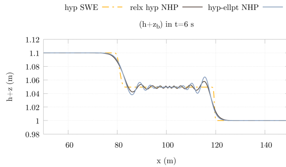
Figure 1: Comparison between a hydrostatic model (SWE), and NHP models (a) and (b) for a dam break simulation.
