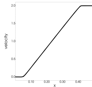
Figure 2: Einfeldt problem, 8 P^{40} elements
