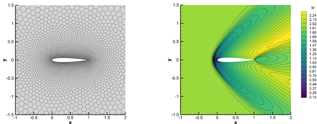
Figure 1: Supersonic flow around NACA 0012 airfoil in a rarefied regime. Mesh and Mach number contours.
