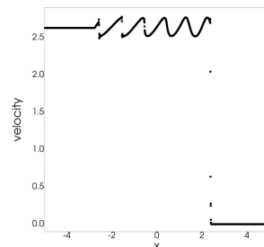
Figure 5: Shu-Osher problem, 400 P^4 elements
