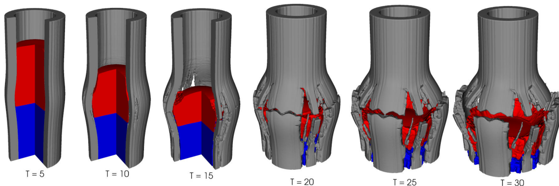
Figure 1: A 3D fracture test run with the model presented. The test depicts two polycarbonate blocks (red and blue) sliding inside a steel cylinder (grey) surrounded by void. As the blocks collide they push the cylinder outwards, eventually leading to fracture. Times shown are in \mu\text{s} .
