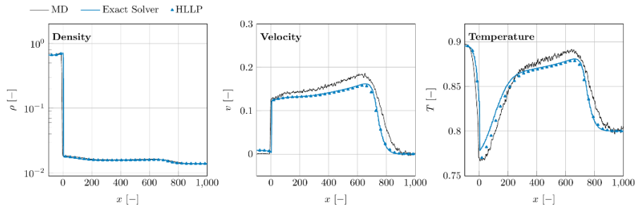
Figure 1: Comparison of macroscopic and molecular dynamics approximate solutions.
