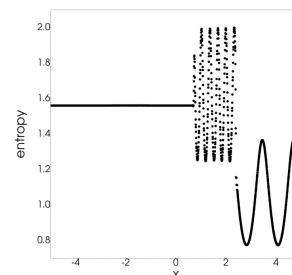
Figure 6: Shu-Osher problem, 400 P^4 elements
