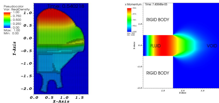
Figure 1: Left: An MHD Riemann problem in a rigid-boundary vessel discretised by means of ghost fluid method. Right: Interaction of plasma with void and a rigid wall using a diffuse interface method.
