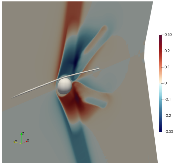
Figure 1: Simulation of Jupiter moon Io and the interaction with its plasma torus. Plot shows the z-component of velocity and the Galileo spacecraft trajectory used for comparison.
