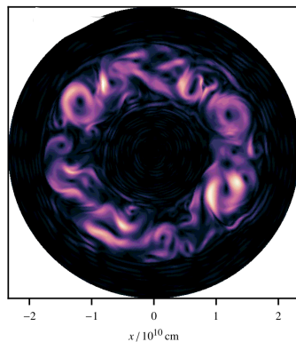
Figure 1: The convective shell in a star, simulated by a well-balanced method that is asymptotic preserving in the low Mach limit
