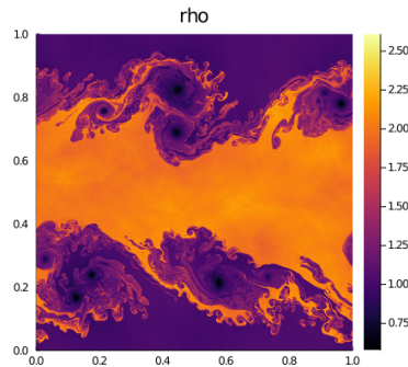
Figure 1: Kelvin-Helmholtz instability.
