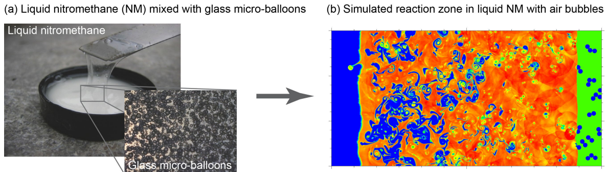
Figure 1: (a) A sample mixture of PMMA-gelled nitromethane and glass micro-balloons (GMBs). (b) Sample simulation result of the reaction-zone structure of a detonation in liquid NM with air-filled bubbles.
