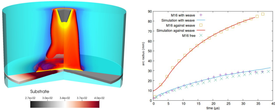
Figure 1: Left: Temperature of arc and substrate for attachment to carbon composite (left half) and aluminium (right half). Right: Validation of the expansion of the arc radius for attachment to carbon composite parallel and perpendicular to the weave direction.
