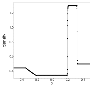
Figure 1: Lax problem, 200 P^4 elements
