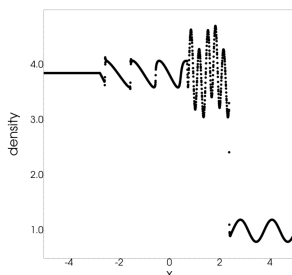
Figure 4: Shu-Osher problem, 400 P^4 elements
