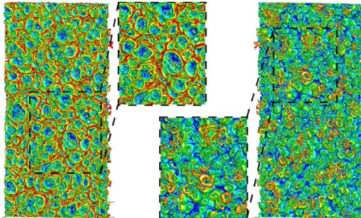
Figure 1: Vortex rings of compressible turbulent mixing flows using 9th-order methods.
