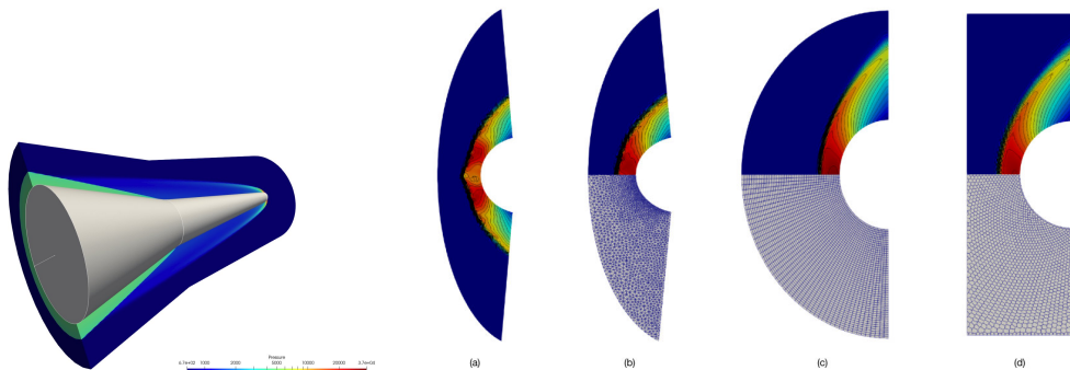
Figure 1: Left: 3D cone flare. Right: half cylinder at Mach 20 for different meshes. The two-point scheme (left most panel) presents some carbuncle phenomenon. The current scheme seems insensitive to it.
