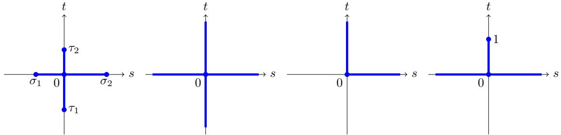
Figure 5.1: Geometric illustrations of box-switching, switching, complementarity, and relaxed reformulated cardinality constraints (from left to right), respectively.
